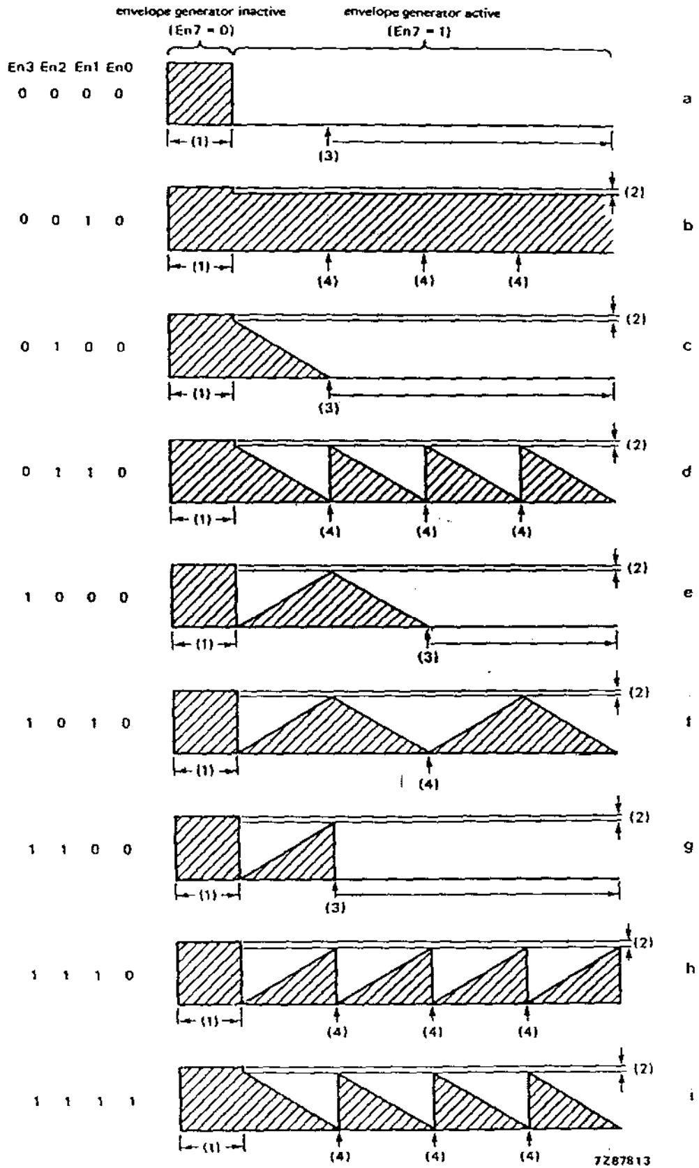
Fig. 5 Envelope waveforms.
